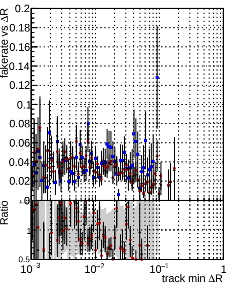
Legend: DQM_V0001_R000000001_Global_cmsswQCD_RECO (blue dots), DQM_V0001_R000000001_Global_mkFitOriginalQCD_RECO (red dots), DQM_V0001_R000000001_Global_mkFitNewQCD_RECO (black dots)
