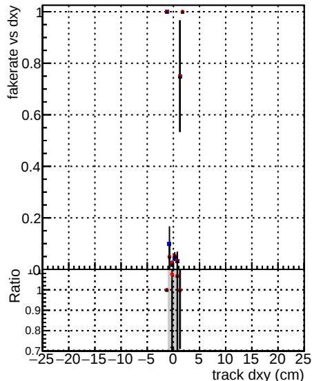
DOM V0001 R0000000001 Global cms-sw QCD RECO DOM V0001 R0000000001 Global mkFit Original QCD RECO DOM V0001 R0000000001 Global mkFit New QCD RECO
