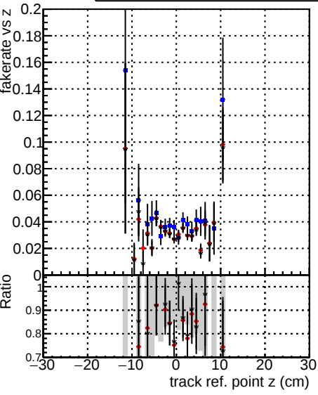
—◆— DQM_V0001_R0000000001 Global cmsswQCD_RECO —●— DQM_V0001_R0000000001 Global mkFitOriginalQCD_RECO —●— DQM_V0001_R0000000001 Global mkFitNewQCD_RECO
