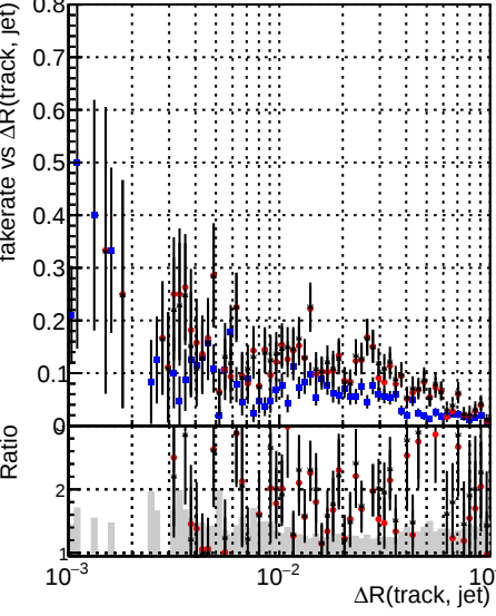
Fake rate vs \Delta R(\text{track, jet}) DQM_V0001_R000000001 Global cmsswQCD_RECO Global mkFitOriginalQCD_RECO Global mkFitNewQCD_RECO
