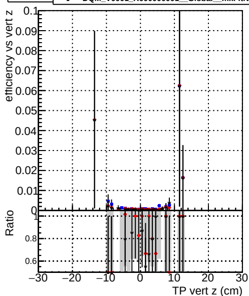
Efficiency Model Fit Reco 0.95 DQM_V0001_R0000000001_Global mkFitOriginalQCD RECO 0.95 DQM_V0001_R0000000001_Global mkFitNewQCD RECO
