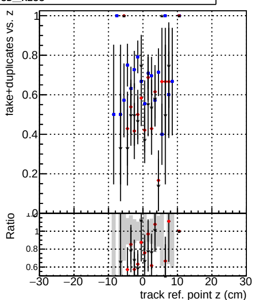
QCD__RECO D__RECO
