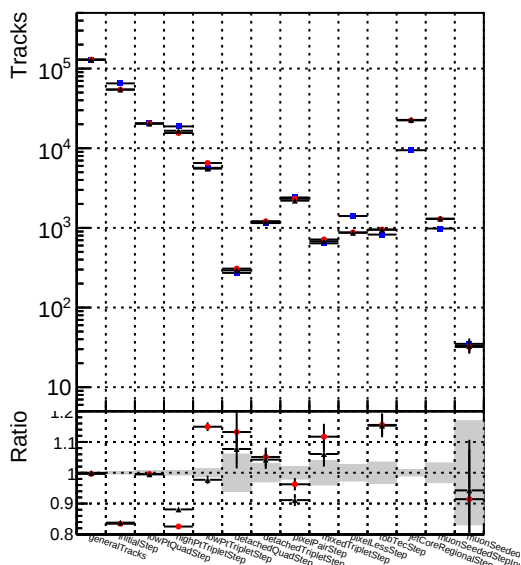
Number of tracks vs collection DQM_V0001_R000000001_Global_cmsswQCD_RECO DQM_V0001_R000000001_Global_mkFitOriginalQCD_RECO DQM_V0001_R000000001_Global_mkFitNewQCD_RECO
