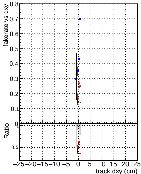
DOM V0001 R0000000001 Global cmsswQCD RECO DOM V0001 R0000000001 Global mktFitOriginalQCD RECO DOM V0001 R0000000001 Global mktFitNewQCD RECO
