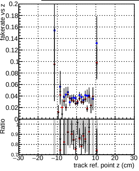
—◆— DQM_V0001_R000000001 Global cmsswQCD_RECO —★— DQM_V0001_R000000001 Global mkFitOriginalQCD_RECO —◆— DQM_V0001_R000000001 Global mkFitNewQCD_RECO
