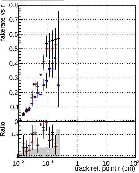
Legend: - Blue line with dots: DQM_V0001_R000000001 Global cmsswQCD RECO - Red line with dots: DQM_V0001_R000000001 Global mkFitOriginalQCD RECO - Black line with dots: DQM_V0001_R000000001 Global mkFitNewQCD RECO
