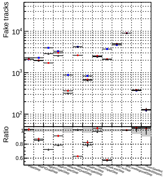
—●— DQM_V0001_R000000001_Global_cmsswQCD_RECO —●— DQM_V0001_R000000001_Global_mkFitOriginalQCD_RECO —●— DQM_V0001_R000000001_Global_mkFitNewQCD_RECO
