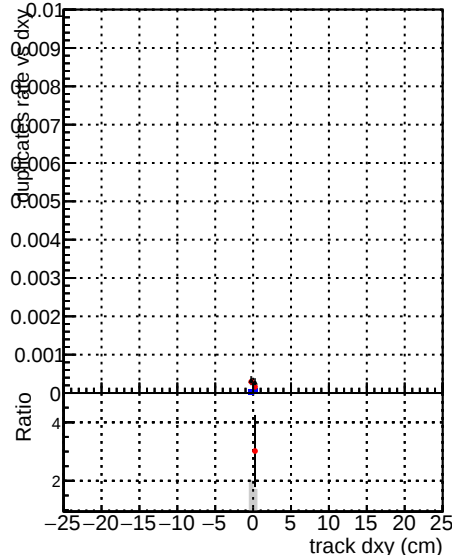
a mkFitOriginal OCD RE a mkFitNew OCD RECO
