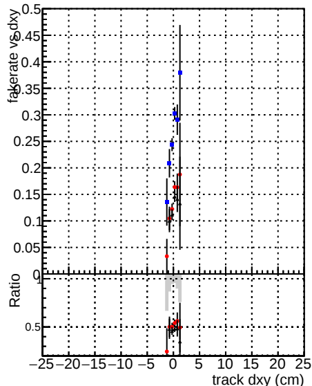
DOM V0001 R0000000001 Global cmsswOCD RECO DOM V0001 R0000000001 Global mktInNewOCD RECO
