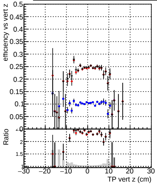
Efficiency vs vert z — DQM_V0001_R000000001_Global_cmsswQCD_RECO — DQM_V0001_R000000001_Global_mkFitOriginalQCD_RECO — DQM_V0001_R000000001_Global_mkFitNewQCD_RECO
