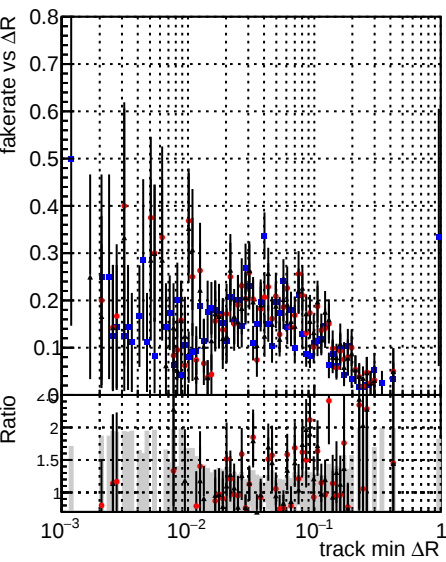
Legend: DQM_V0001_R000000001_Global_cmsswQCD_RECO (blue stars), DQM_V0001_R000000001_Global_mkFitOriginalQCD_RECO (red stars), DQM_V0001_R000000001_Global_mkFitNewQCD_RECO (black stars)
