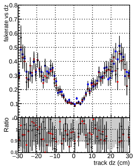
DOM V0001 DOM V0001 RECO Global mktNewQCD RECO DOM V0001 DOM V0001 RECO Global mktNewQCD RECO
