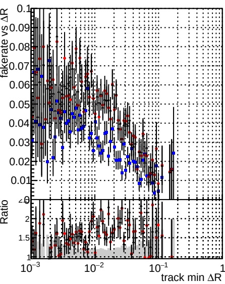
Legend: DQM_V0001_R000000001 Global cmsswQCD_RECO, DQM_V0001_R000000001 Global mkFitOriginalQCD_RECO, DQM_V0001_R000000001 Global mkFitNewQCD_RECO
