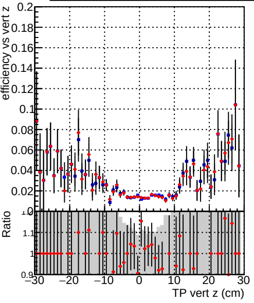
Efficiency vs TP vert z (cm) Legend: DQM_TT_mkFit_ORIG (blue diamonds), DQM_TT_mkFit_MODIF (red diamonds)
