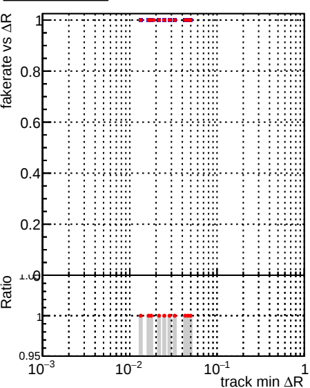
Fake rate vs \Delta R(\text{track, jet}) Legend: \square DQM_TT_mkFit_ORIG \bullet DQM_TT_mkFit_MODIF
