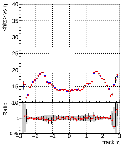
mean hits — DQM_TT_mkFit_ORIG — DQM_TT_mkFit_MODIF
