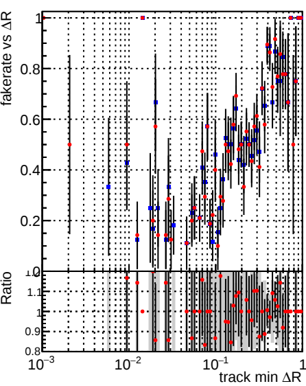
Fake rate vs \Delta R(\text{track, jet}) Legend: DQM_TT_mkFit_ORIG (blue squares), DQM_TT_mkFit_MODIF (red circles)
