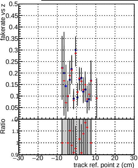
Fake rate vs v DQM_TT_mkFit_ORIG DQM_TT_mkFit_MODIF
