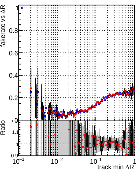
Fake rate vs \Delta R(\text{track, jet}) Legend: \blacksquare DQM_TT_mkFit_ORIG \bullet DQM_TT_mkFit_MODIF
