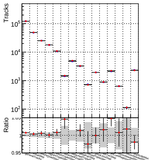
Number of tracks vs collection Legend: DQM_TT_mkFit_ORIG (Blue line with circles) DQM_TT_mkFit_MODIF (Red line with circles)
