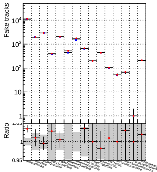
Number of tracks vs collection Legend: DQM_TT_mkFit_ORIG (Blue line with circles) DQM_TT_mkFit_MODIF (Red line with circles)
