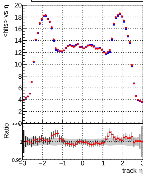
mean hit — DQM_TT_mkFit_ORIG — DQM_TT_mkFit_MODIF
