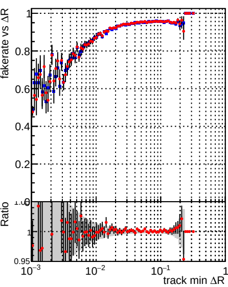
Legend: DQM_TT_mkFit_ORIG (blue squares), DQM_TT_mkFit_MODIF (red circles)
