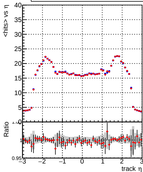
mean hits — DQM_TT_mkFit_ORIG — DQM_TT_mkFit_MODIF
