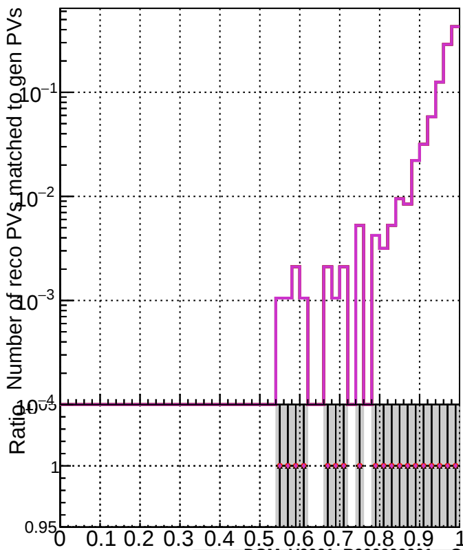
RecoPVAssoc2GenPVMatched_Purity
