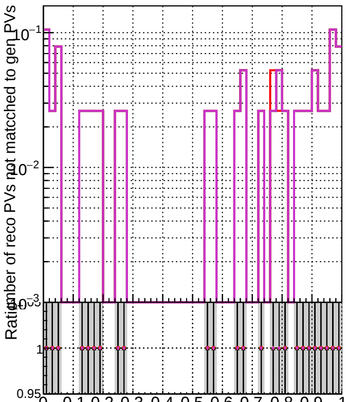
RecoPVAssoc2GenPVNotMatched_missing
