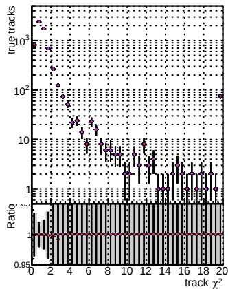
N of reco track vs. BOM V0001 R0000000001 Global \chi^2 MISSINGNER RECO BOM V0001 R0000000001 Global \chi^2 INOMER RECO
