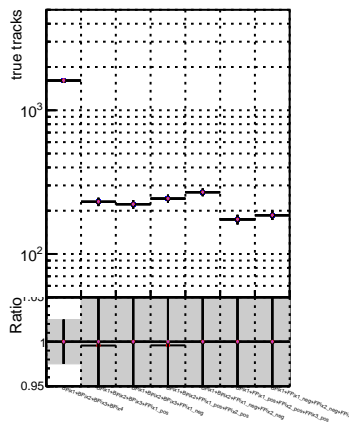
N of reco track vs. DOM V0001 R0000000001 Global m-EISSINER-RECO DOM V0001 R0000000001 Global m-EISSINER-RECO DOM V0001 R0000000001 Global m-EISSINER-RECO
