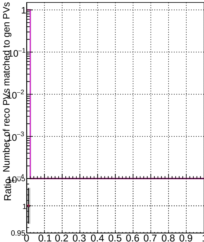
RecoPVAssoc2GenPVMatched_Purity
