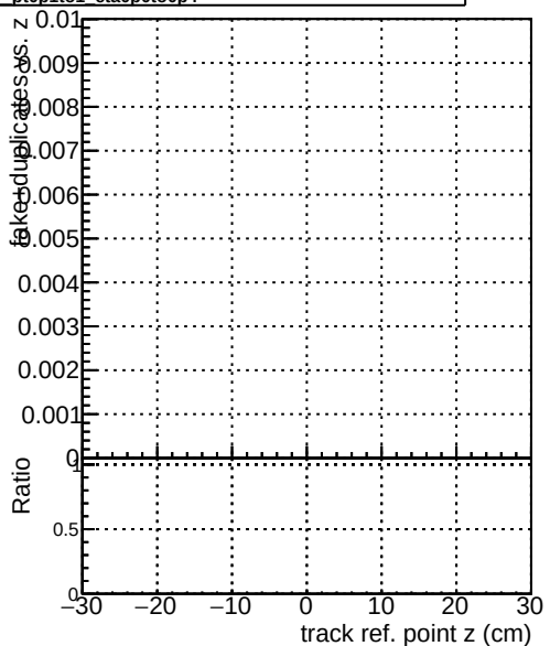
pt0p1to1-eta0p0to0p4 pt0p1to1-eta0p0to0p4 pt0p1to1-eta0p0to0p4
