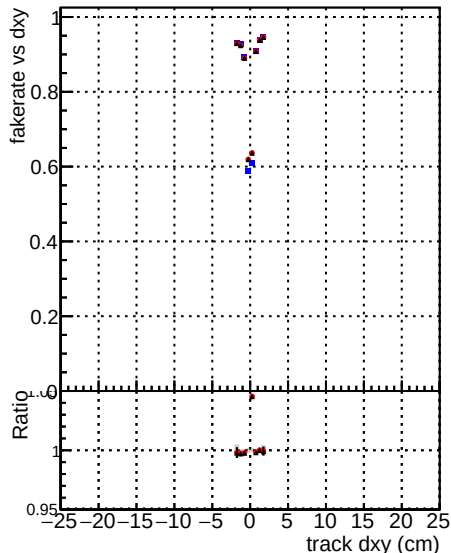
Legend for Fake rate vs d, Duplicates Rate vs Dxy, and Pileup rate vs dxy: Global cmssw1000time RECO Global mktNewBmsAd1000time RECO Global mktNewBmsAd1000time RECO
