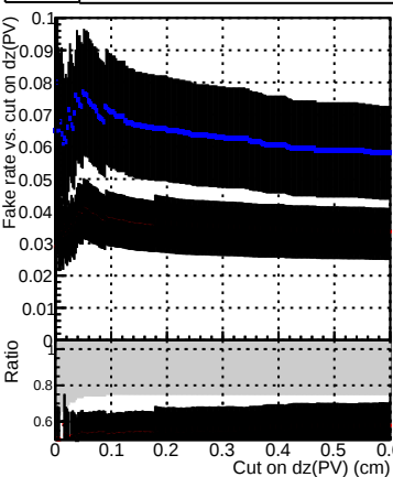
Fake rate
