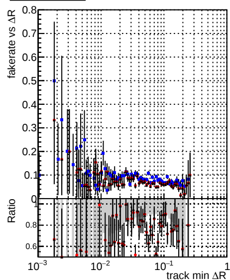
—●— DQM_V0001_R000000001 Global cmssw1000time RECO —●— DQM_V0001_R000000001 Global mkFitNewOLD1000time RECO —●— DQM_V0001_R000000001 Global mkFitNewBinsAdj1000time RECO
