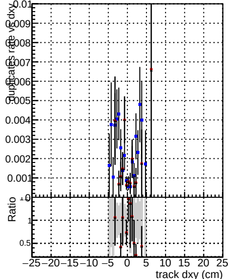
DOM V0001 R0000000001 Global cms-sw-1000time RECO DOM V0001 R0000000001 Global mkFitNewBinsAd-1000time RECO
