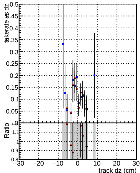
Fake rate vs dz Legend: DOM V0001 R0000000001 Global cms-sw1000time RECO DOM V0001 R0000000001 Global mktFitNewBmsAd1000time RECO DOM V0001 R0000000001 Global mktFitNewBmsAd1000time RECO
