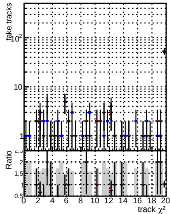
N of fake tracks vs normalized \chi^2
