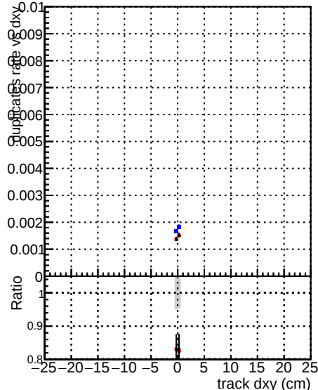
DOM V0001 R0000000001 Global cms-sw1000time RECO DOM V0001 R0000000001 Global mktFitNewBinsAd1000time RECO
