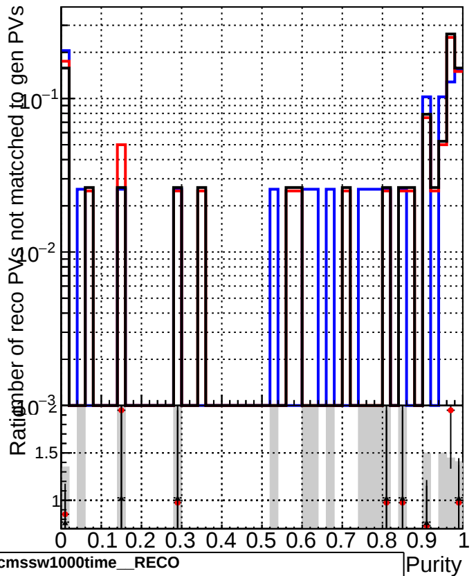
RecoPVAssoc2GenPVNotMatched_Purity
