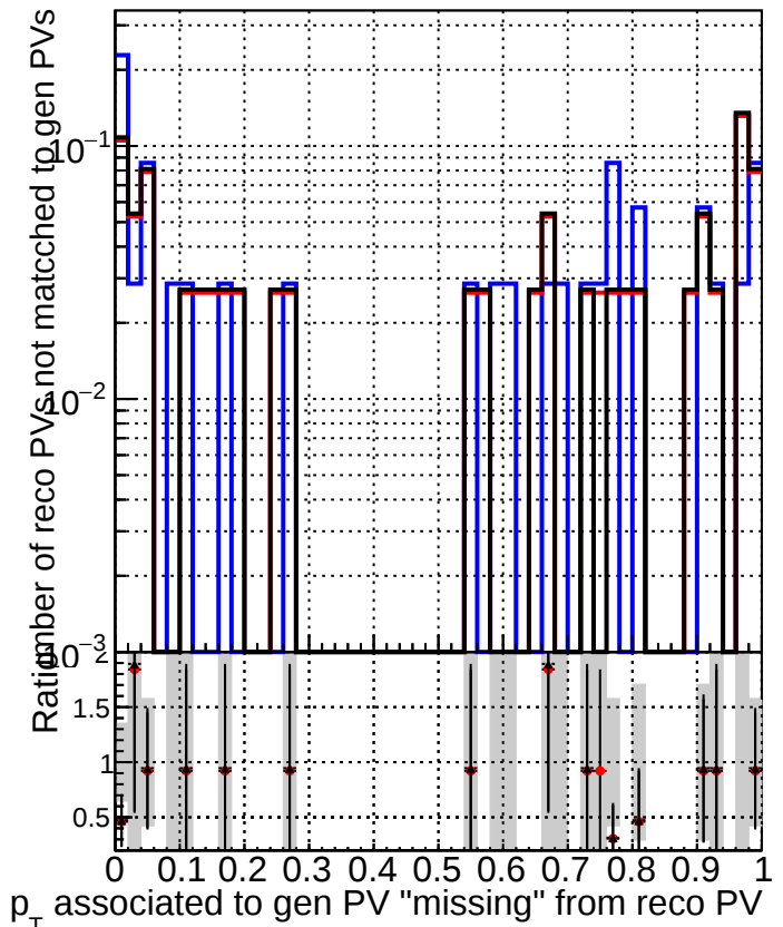
RecoPVAssoc2GenPVNotMatched_missing
