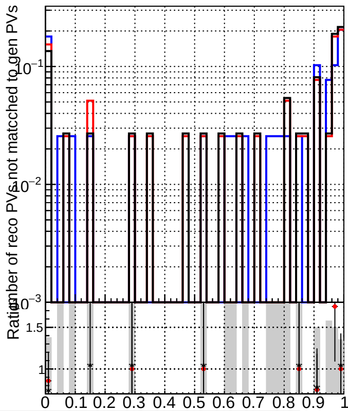
RecoPVAssoc2GenPVNotMatched_Purity
