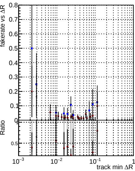
Fake rate vs ΔR(track, jet) DQM_V0001_R000000001 Global cmssw1000time RECO DQM_V0001_R000000001 Global mkFitNewOLD1000time RECO DQM_V0001_R000000001 Global mkFitNewBinsDC1000time RECO
