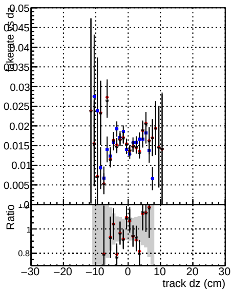
Configuration Global cmssw1000time RECO DOM V0001 R0000000001 Global cmssw1000time RECO DOM V0001 R0000000001 Global mkFitNewOLD1000time RECO DOM V0001 R0000000001 Global mkFitNewBInsDC1000time RECO
