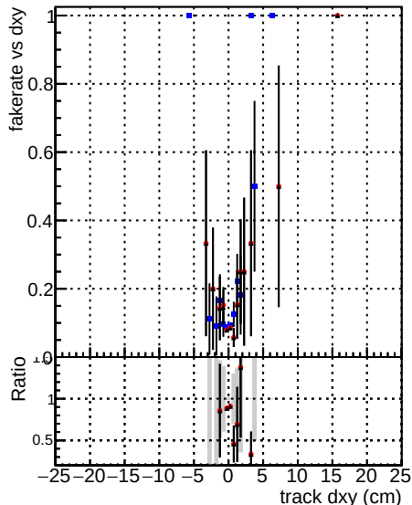
DOM V0001 R0000000001 Global cmssw1000time RECO DOM V0001 R0000000001 Global mkFitNewOld1000time RECO DOM V0001 R0000000001 Global mkFitNewBmsDC1000time RECO
