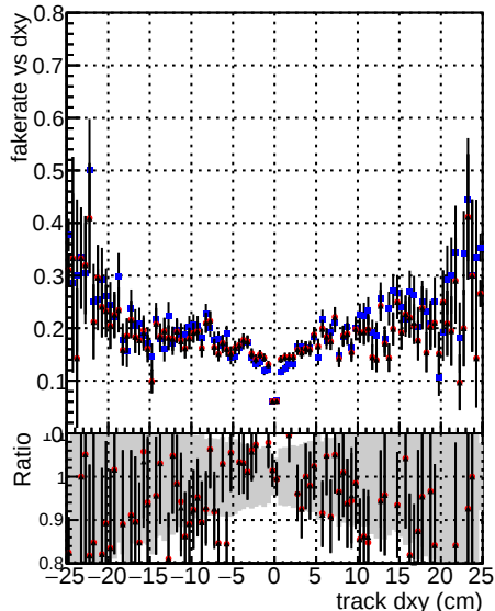
Model Dataset Configuration Global cmssw1000time RECO Fake rate vs d DOM V0001 R0000000001 Global cmssw1000time RECO DOM V0001 R0000000001 Global mkFitNewOLD1000time RECO DOM V0001 R0000000001 Global mkFitNewBindsDC1000time RECO
