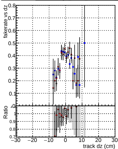
DOM V0001 R0000000001 Global cms-sw1000time RECO DOM V0001 R0000000001 Global mkFitNewBmsDC1000time RECO DOM V0001 R0000000001 Global mkFitNewBmsDC1000time RECO
