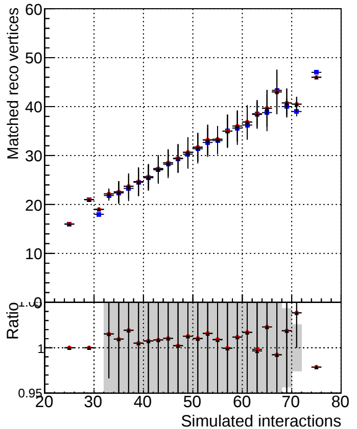
MatchedRecoVtx_vs_GenVtx
