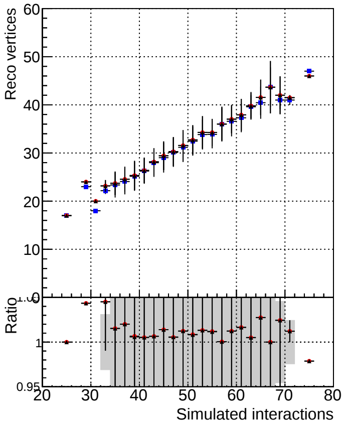
RecoVtx_vs_GenVtx
