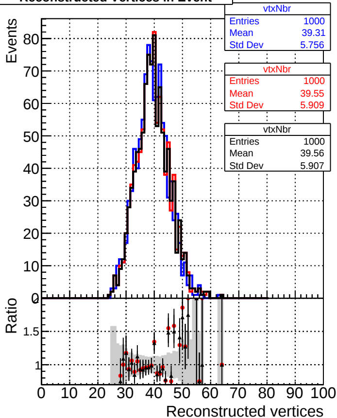
Reconstructed Vertices in Event
