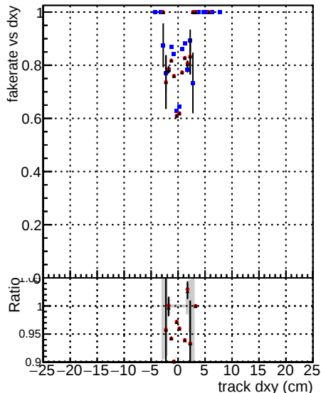
Legend for all plots: DOM V0001 R0000000001 Global cms-sw1000time RECO DOM V0001 R0000000001 Global mktFitNewBinsDC1000time RECO
