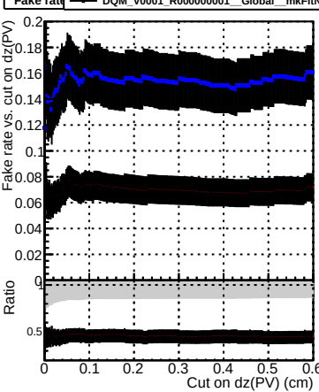
Fake rate
