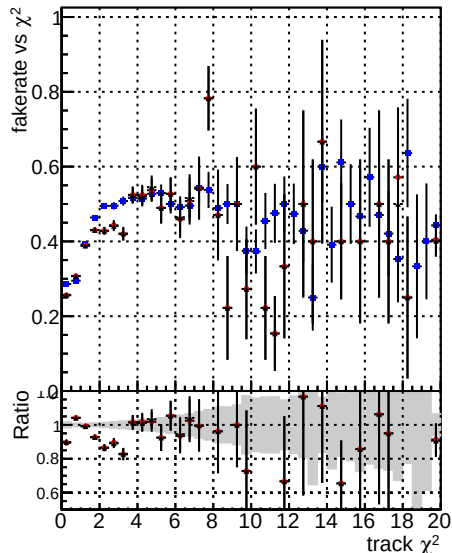
Fake rate vs. Legend Global cmssw1000time RECO Blue line DOM_V0001_R0000000001 cmssw1000time RECO Red line DOM_V0001_R0000000001 mkFitNewOL.D1000time RECO Black line DOM_V0001_R0000000001 mkFitNewBmsDC1000time RECO
